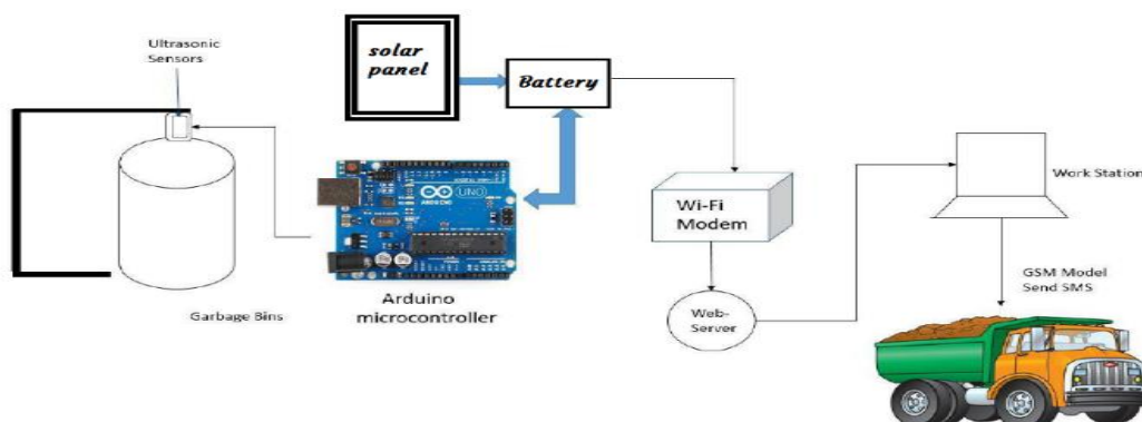
Figure.2 Block Diagram of system
